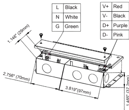
Wiring/Open View
