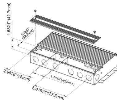
Open View
