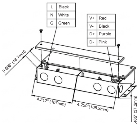
Wiring/Open View
