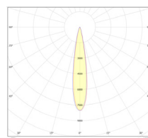
Beam Angle:18°
