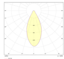
Beam Angle:50°
