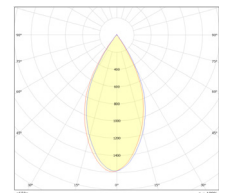
Beam Angle:50°
