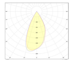
Beam Angle:55°
