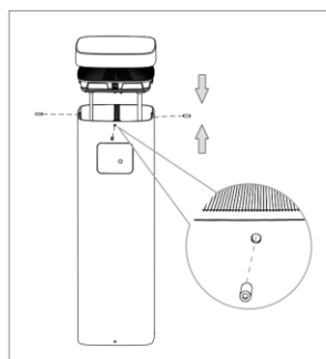
8. Fix the bollard head and bollard tube
